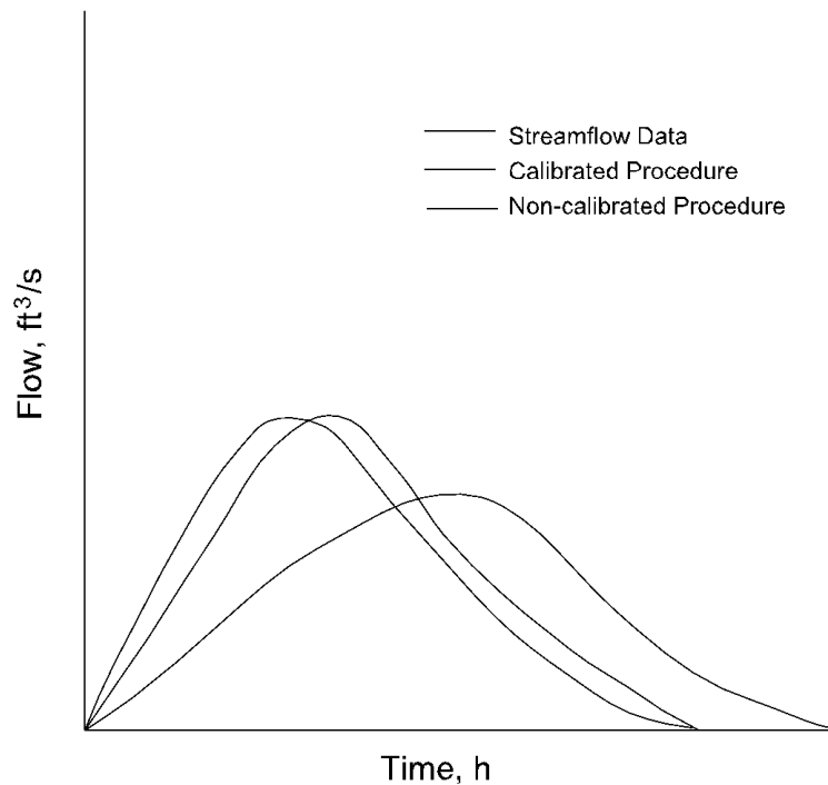
Figure 7.3 Calibrated Hydrograph
