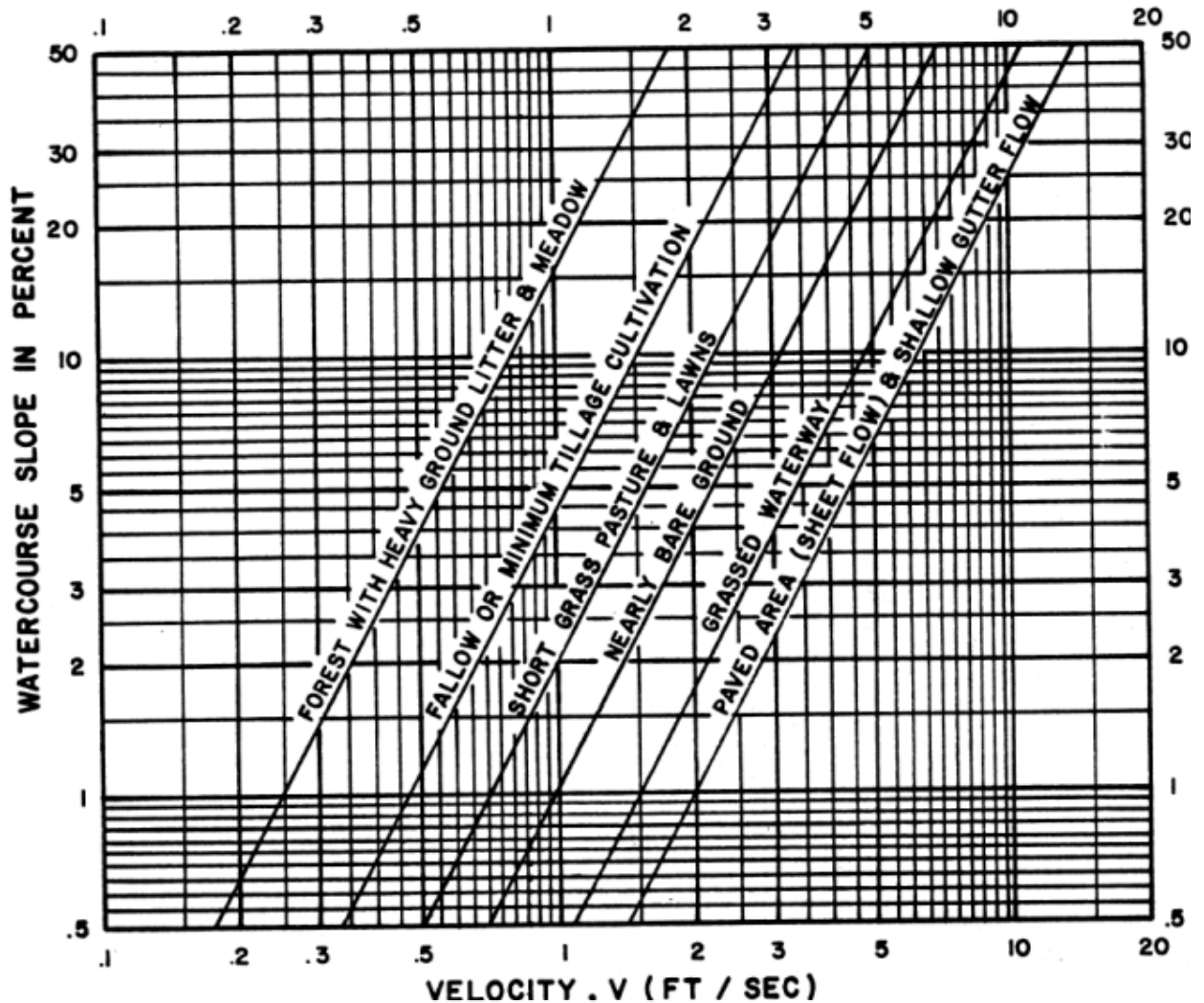
Figure 7.2 Velocities for Estimation of Time of Concentration
